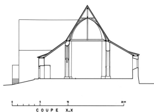
Coupe transversale. Repro. Guy Artur, Repro. Norbert Lambart IVR53_19843500220P
