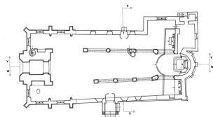
Plan au sol. Repro. Guy Artur, Repro. Norbert Lambart IVR53_19843500224P
