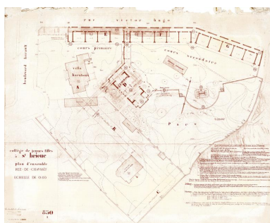
Plan masse, 1934. Dess. Georges-Robert Lefort IVR53_20182206103A0
