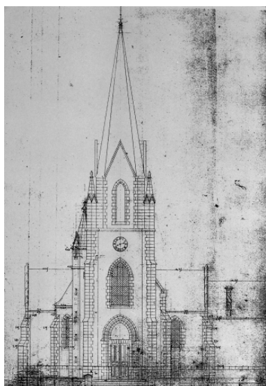
Elévation ouest. Autr. Arthur Regnault IVR53_19973500302X
