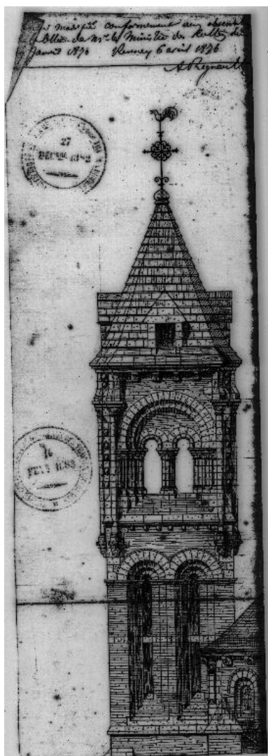
Plan du clocher Repro. Guy Artur IVR53_19813500310P
