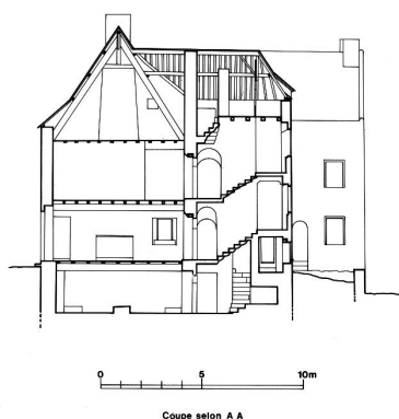
Coupe transversale Repro. Guy Artur, Repro. Norbert Lambart IVR53_19882900217P
