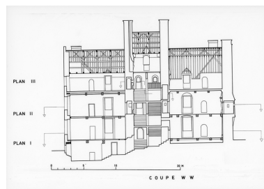
Coupe V-W Phot. Guy Artur, Autr. P Boutroux IVR53_19762200374P
