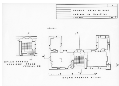
Plan Phot. François Dagorn IVR53_19762200088P
