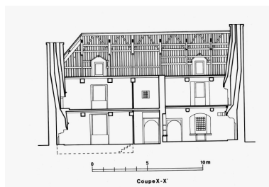
Coupe XX'. Phot. Guy Artur, Phot. Norbert Lambart IVR53_19873500494P
