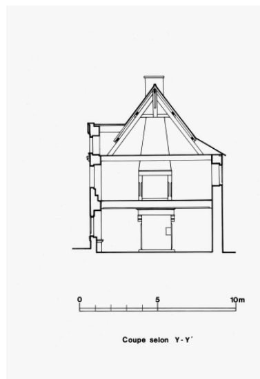
Coupe selon YY'. Phot. Guy Artur, Phot. Norbert Lambart IVR53_19873500492P
