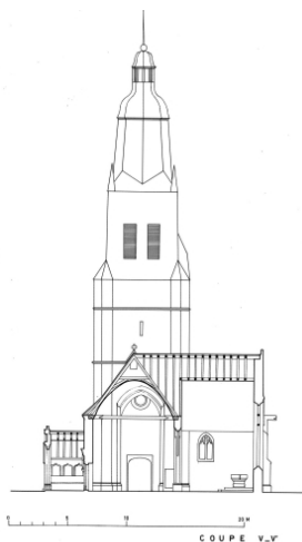
Coupe V-V', 1968. Phot. Guy Artur, Phot. Norbert Lambart, Autr. A. Corre, Autr. Delournay R IVR53_19903500075P
