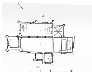
Plan au sol, 1968. Phot. Guy Artur, Phot. Norbert Lambart, Autr. A. Corre, Autr. Delournay R IVR53_19903500076P
