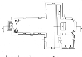
Plan au sol. Repro. Norbert Lambart IVR53_19843501619P
